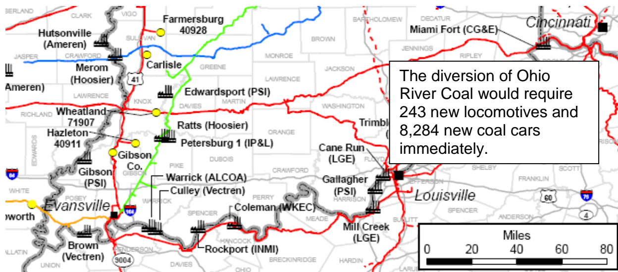
Figure 17. CSX IN-IL-Ohio River Regional Railroad Network. 8
