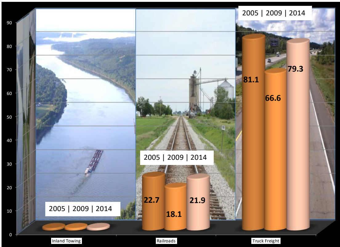
Figure 21. Ratio of Fatalities per Million Ton-Miles versus Inland Towing (2001–05, 2001–09, and 2001–14).
