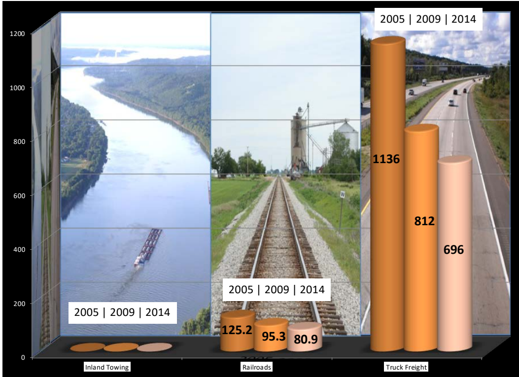
Figure 22. Ratio of Injuries per Million Ton-Miles versus Inland Towing (2001–05, 2001–09, and 2001–14).
