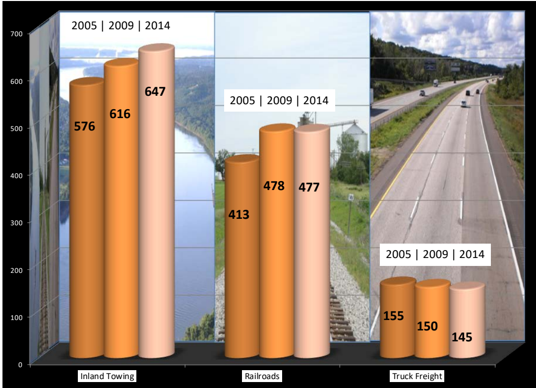
Figure 20. Comparison of Fuel Efficiency—2005, 2009, and 2014.
