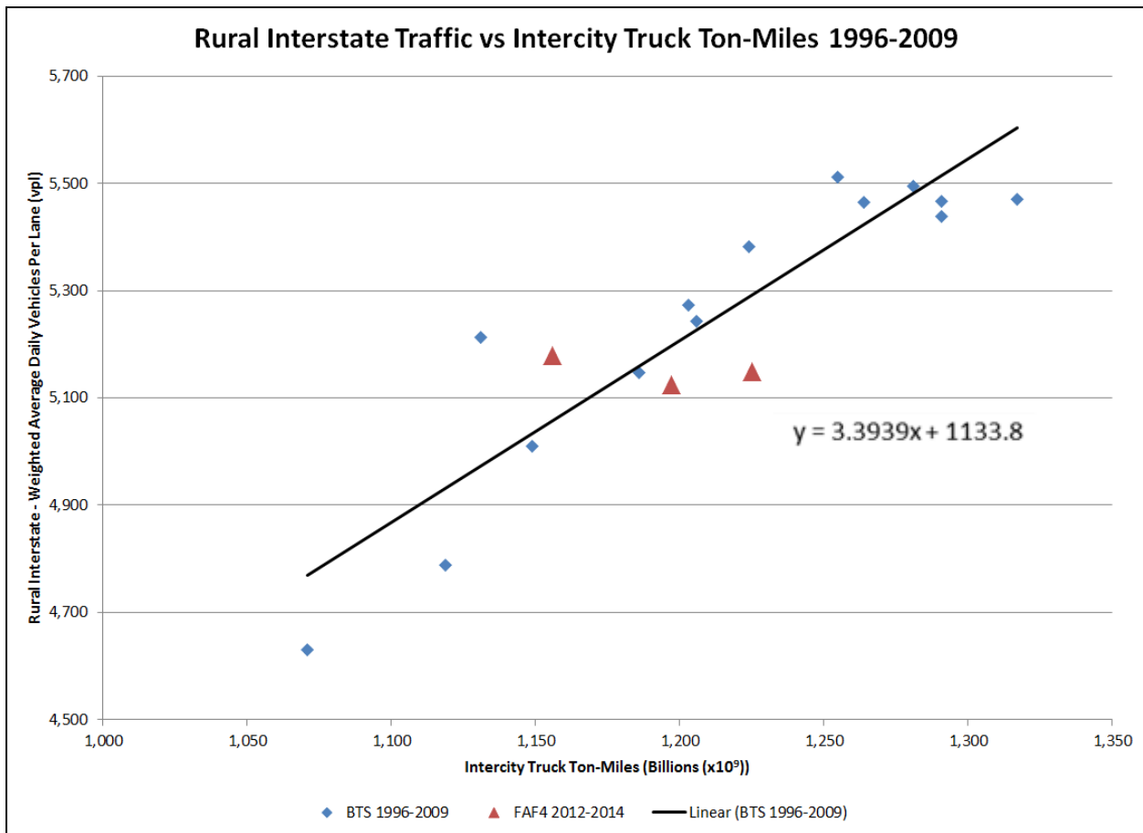
Figure 4. Average Daily Vehicles per Lane of Rural Interstate vs. Intercity Truck Ton-Miles.
