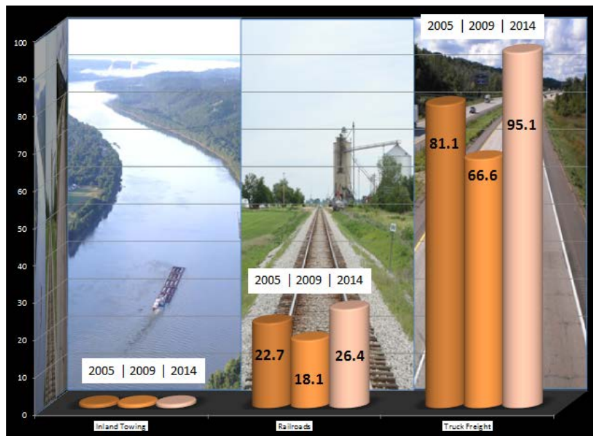
Figure ES-8. Ratio of Fatalities per Million Ton-Miles versus Inland Towing (2001–05, 2001–09, and 2001–14).
