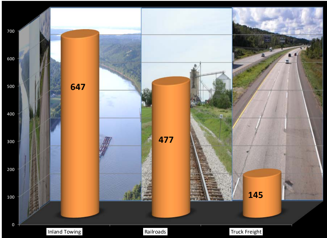
Figure 12. Comparison of Fuel Efficiency—2014.
