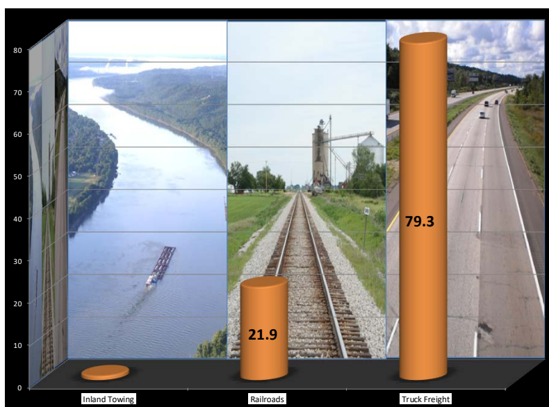
Figure ES-6. Ratio of Fatalities per Million Ton-Miles versus Inland Towing—2001–2014.
