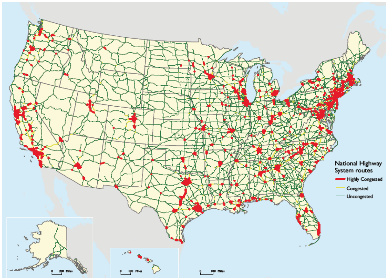
Figure 6. Peak-Period Congestion on High-Volume Truck Portions of the National Highway System (2011) (12).
