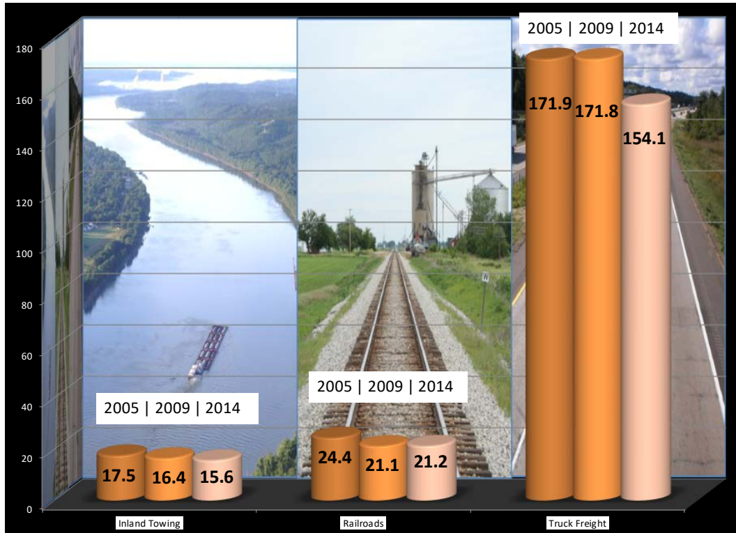
Figure ES-3. Metric Tons of GHG per Million Ton-Miles (2005, 2009, and 2014).
